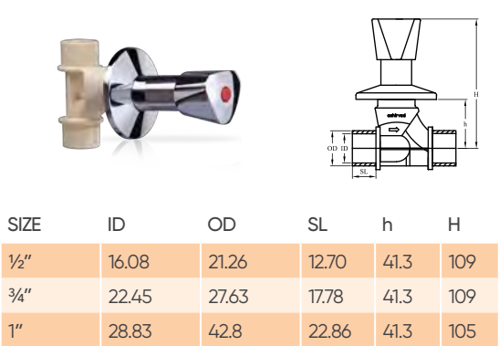
CPVC CONCEALED DIVERTER – SHOWER & SPOUT
