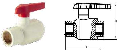
BALL VALVE WITH BRASS THREADED (TWO SIDE)
