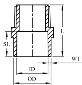
MALE ADAPTER PLASTIC THREADED - MAPT
