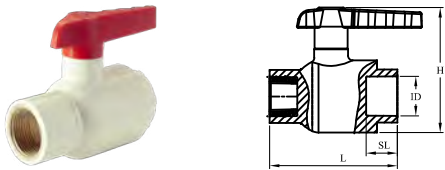
BALL VALVE WITH BRASS THREADED (ONE SIDE)
