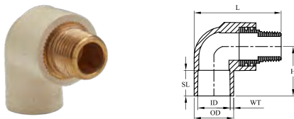
BRASS ELBOW - MABT
