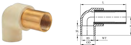
BRASS ELBOW - LONG
