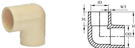
ELBOW 90°
