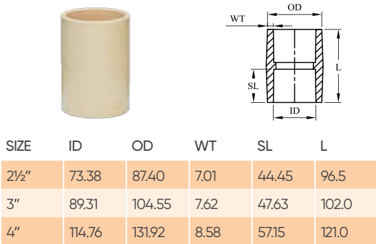
COUPLER (SCH 40)
