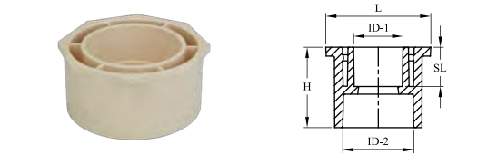
BUSHINGS (SCH 40 AND 80)
