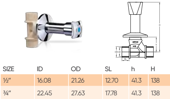
LONG CONCEALED VALVE
