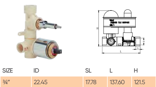
CPVC CONCEALED DIVERTER – SHOWER
