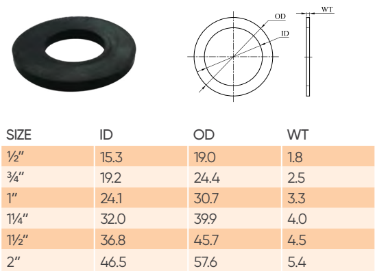
TANK NIPPLE WASHER
